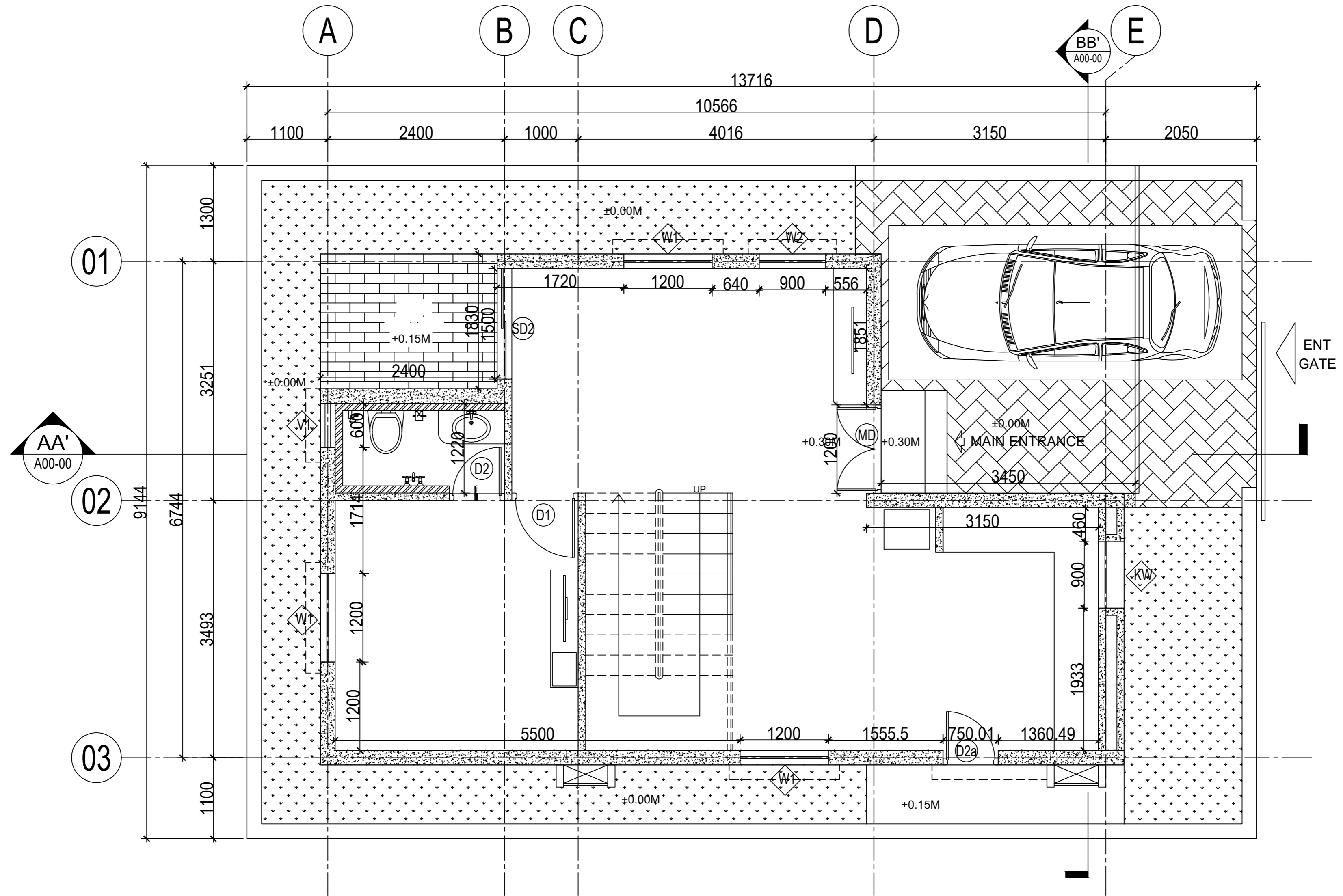
1 A00-00 1:100 GROUND FLOOR PLAN
